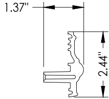
2 INTERIOR FRAME INTERCEPT HARMONY BLIND (HP POLYPROPYLENE)
