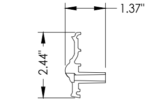
1 EXTERIOR FRAME INTERCEPT HARMONY BLIND (HP POLYPROPYLENE)
