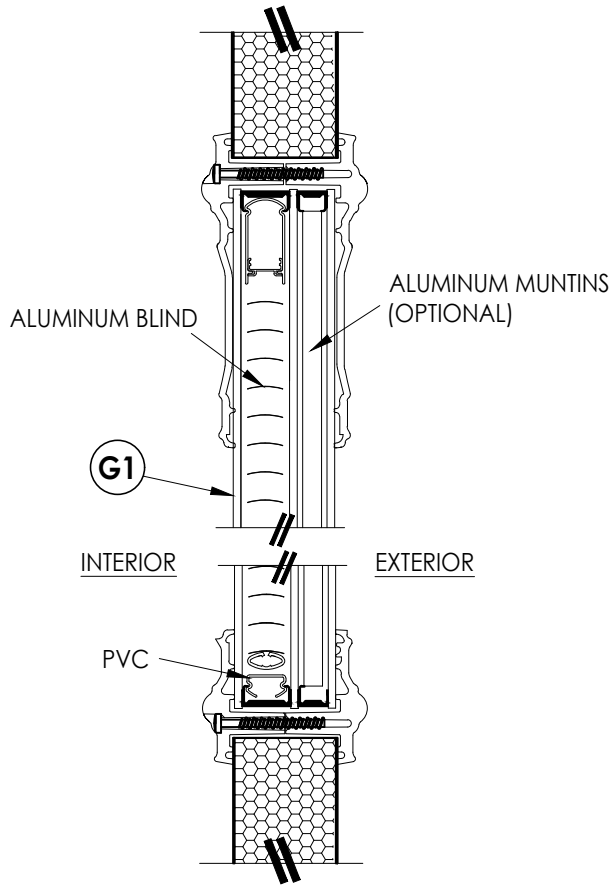
2 VERTICAL CROSS SECTION 2
