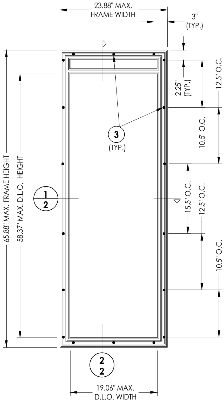
TRIPLE-GLAZED HARMONY BLIND FRAME SYSTEM HP Polypropylene
