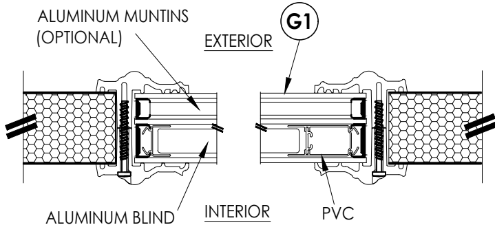
1 HORIZONTAL CROSS SECTION 2
